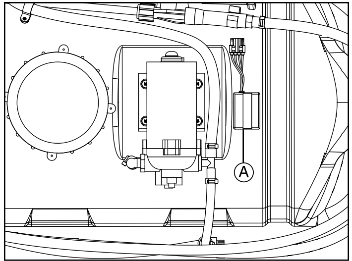
Figure 2 - 15 and 25 gal tank installation
